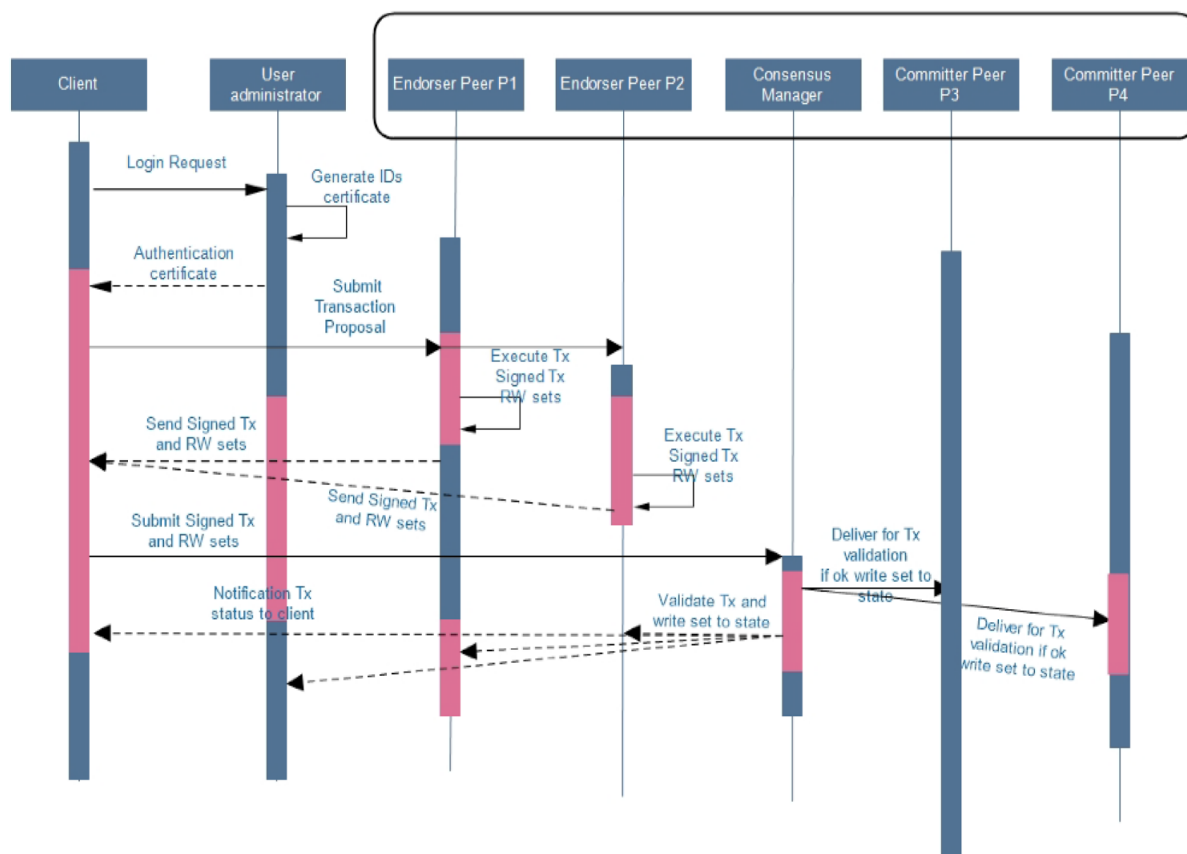
Figure 2: Transaction Execution Procedure
