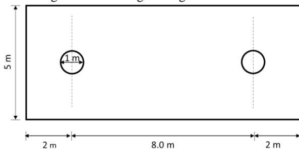
Fig. 1. Existing Foundation before Retrofitting.
