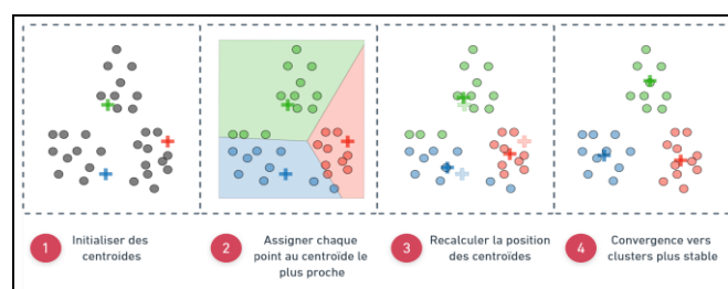
Fig. 4. Illustration of the K-Means Algorithm.
