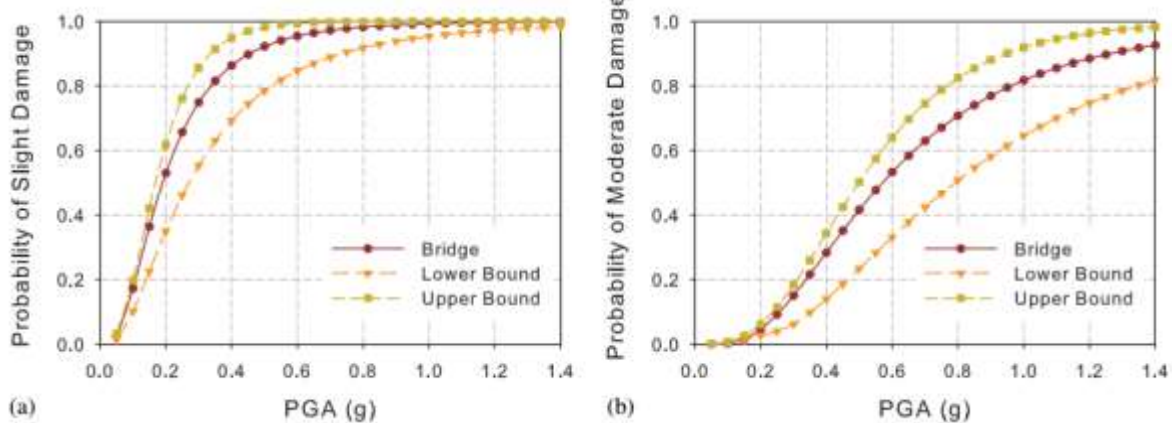
Fig13. Bridge and system fragility bounds for: (a) slight damage; and (b) moderate damage.
