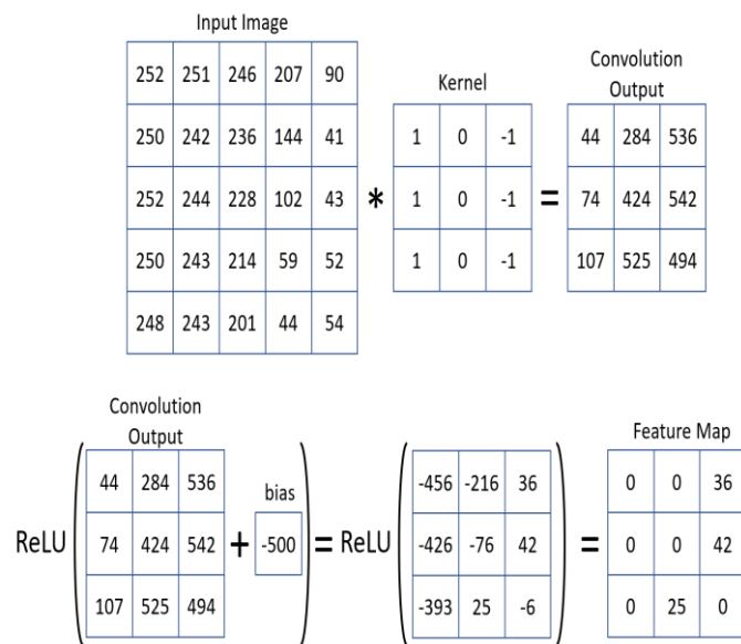
Fig. 9. ReLU function visual representation after convolution
