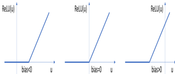
Fig. 8. ReLU process of Graph
