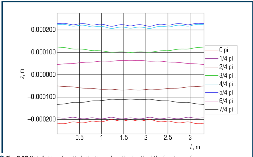
Fig. 8.19 Distribution of vertical vibrations along the length of the forming surface
