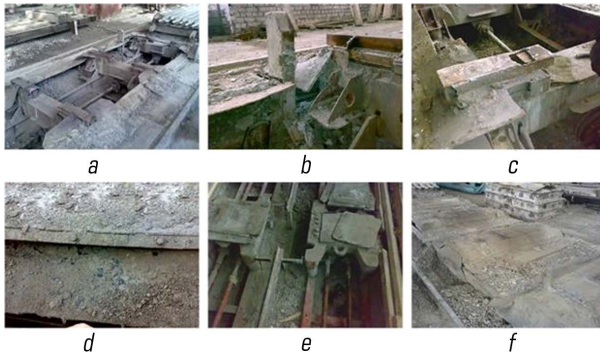
○ Fig. 7.18 Photo fixation of failures of the working bodies of vibration platforms: a – failure of vibration plates; b – deformation of the limiters; c – damage to the contact platform; d – damage to the protective casing; e – damage to vibration plates; f – blockage of the vibration platform
