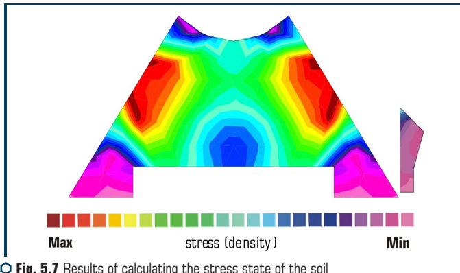
○ Fig. 5.7 Results of calculating the stress state of the soil mass under the pipeline for typical experimental plans
