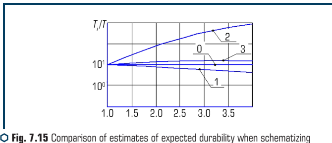
○ Fig. 7.15 Comparison of estimates of expected durability when schematizing by different methods: 0 – bursting; 1 – maximums; 2 – swings; 3 – full cycles
