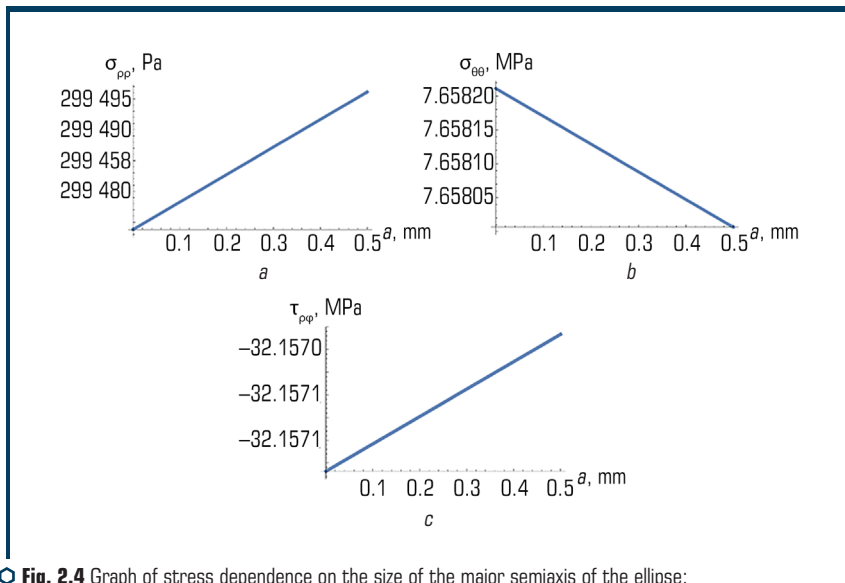
○ Fig. 2.4 Graph of stress dependence on the size of the major semiaxis of the ellipse: a – \sigma\rho – a ; b – \sigma\theta – a ; c – \tau\rho\phi – a
