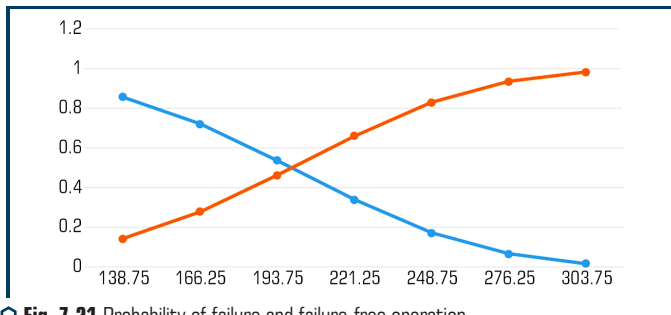
Fig. 7.21 Probability of failure and failure-free operation
