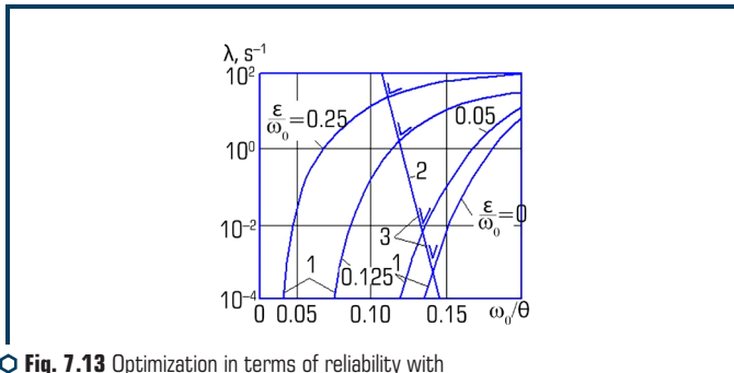
○ Fig. 7.13 Optimization in terms of reliability with a narrow-linear initial impact
