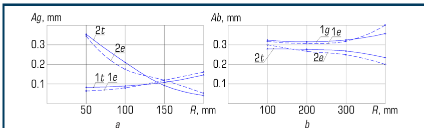
Fig. 4.9 Comparison of theoretical and experimental values of the amplitude: a – horizontal vibrations of the bottom and shell, depending on the radius; b – vertical vibrations of the bottom and shell for the mixture G=30 s
