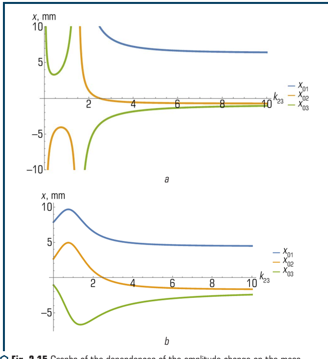
Fig. 2.15 Graphs of the dependences of the amplitude change on the mass ratio k_{23} at different frequency ranges: a - \omega_0 = 104.67 rad/s; b - \omega_0 = 314 rad/s
