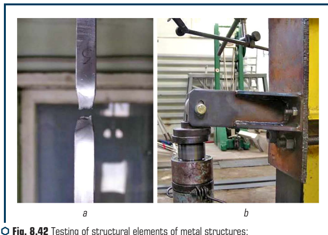
Fig. 8.42 Testing of structural elements of metal structures: a – tensile welded joint; b – bracket test
