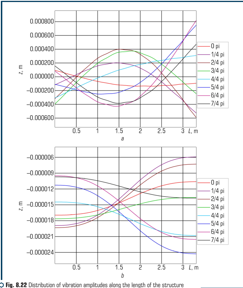
Fig. 8.22 Distribution of vibration amplitudes along the length of the structure for one period of vibration (angle = 60^\circ ): a – X axis; b – Y axis
