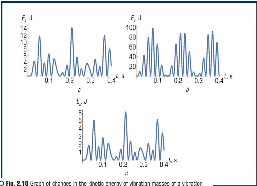
Fig. 2.10 Graph of changes in the kinetic energy of vibration masses of a vibration jaw crusher: a – first mass; b – second mass; c – third mass
