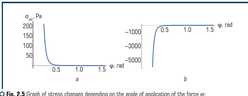
○ Fig. 2.5 Graph of stress changes depending on the angle of application of the force: a – \sigma\rho – \varphi ; b – \tau\rho\phi – \varphi
