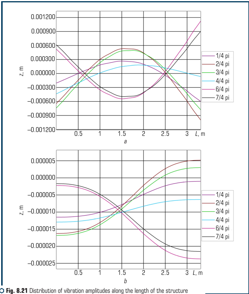
Fig. 8.21 Distribution of vibration amplitudes along the length of the structure for one period of vibration (angle = 90^\circ ): a – X axis; b – Y axis
