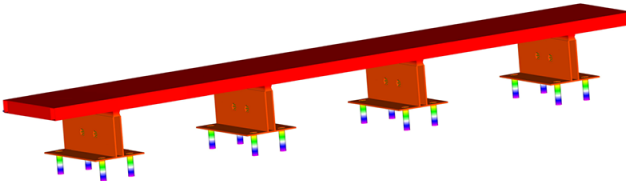
○ Fig. 8.14 Vibration mode (Mode 8, f=4,10 Hz)
