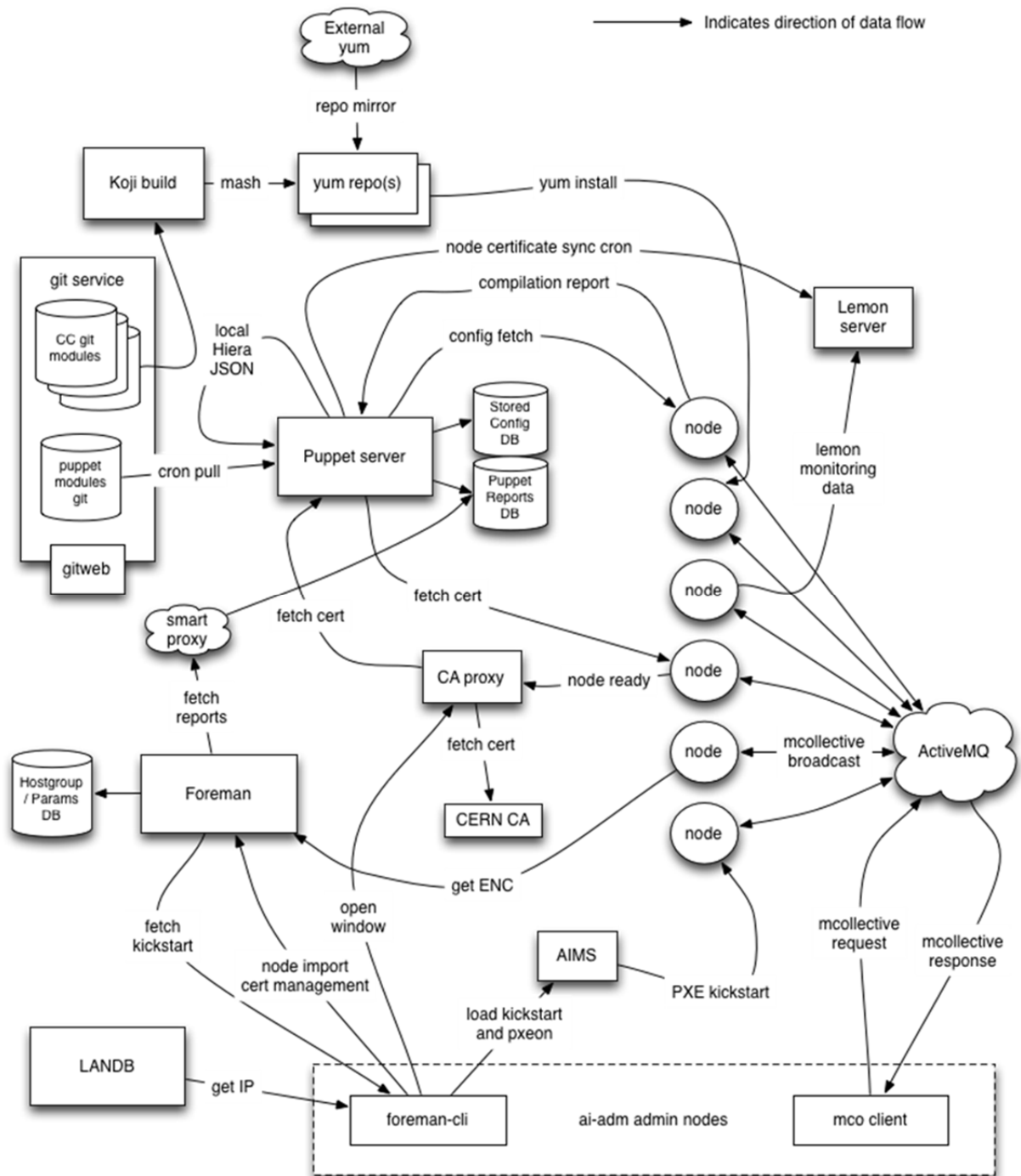
Figure 2 Configuration Management Data Flow
