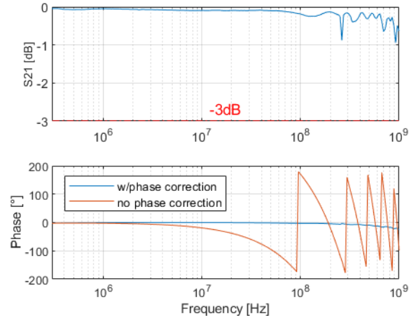
Fig. 3. Test bench frequency response amplitude and phase.
