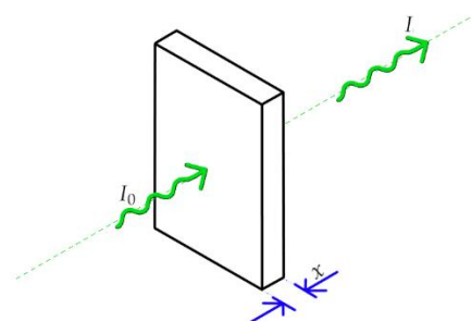
Figure 12: Representation of absorption of a unit of flux through a thickness of ' x '
