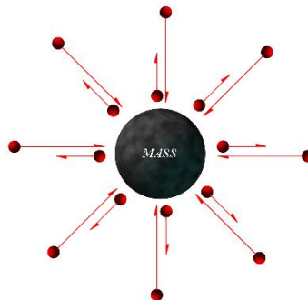
Figure 2: A small fraction of flux is absorbed in mass, resulting in a flux exit energy being reduced from the incident flux.
