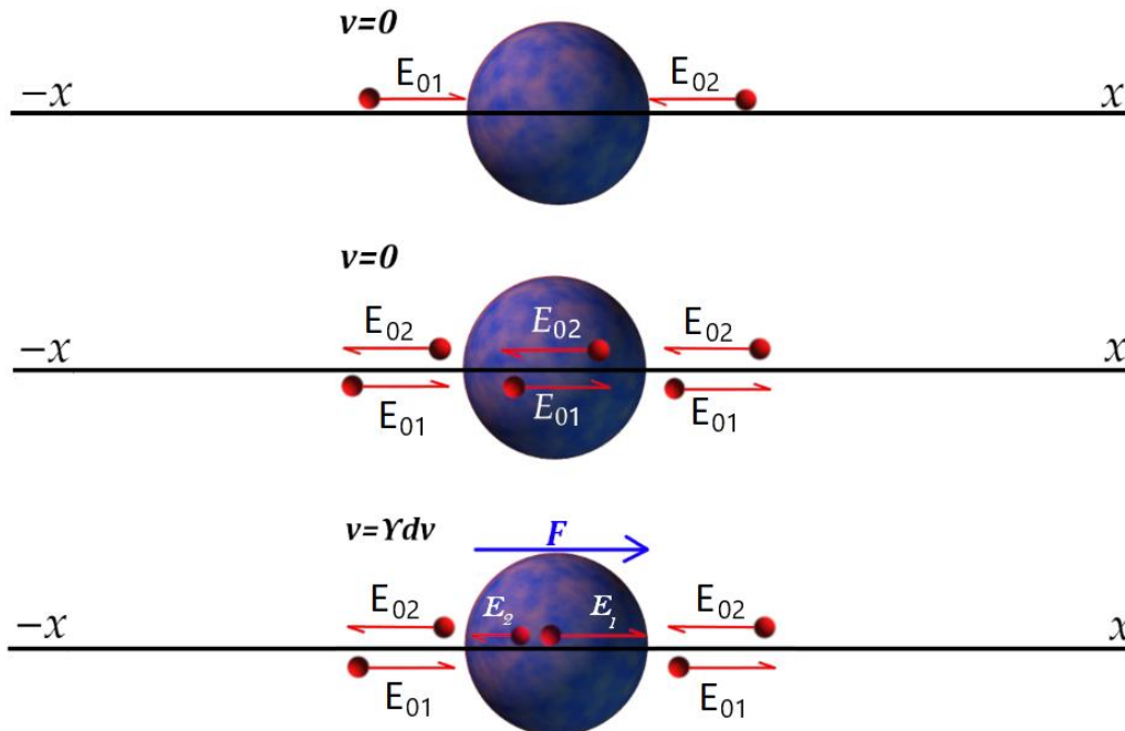
Figure 4: From an observer point of view, the flux particles in the mass are transformed when the mass is accelerated due to an external force. Top picture: the flux is shown around the mass as equal \pm E_{0i} . Mid picture: the mass is transparent to the flux and \pm E_{0i} is also within the mass. Bottom picture: The mass is accelerated and the particles within are transformed to E_1 and E_2 , blue-shifted and red-shifted respectively. The surrounding particles remain undisturbed to an external observer. (arrow lengths are not to scale, and represent vector strengths, not particle wavelengths)
