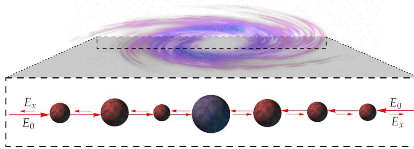
Figure 16: Representation of flux absorption in a spiral galaxy disc, viewed side-on, shows diminishing flux from each side until out the other side.
