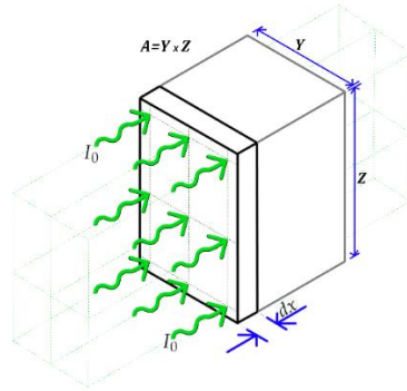
Figure 13: Representing absorption of a measure of flux across an area A, through a distance x
