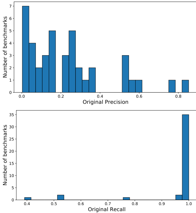
Figure 5: Precision and recall for 41 test programs.
