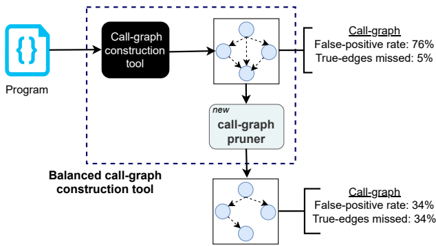
Figure 1: Overview of our technique
