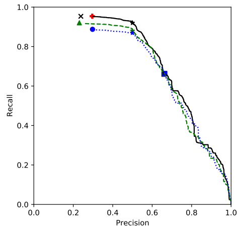
Figure 6: Precision and recall after call-graph pruning.
