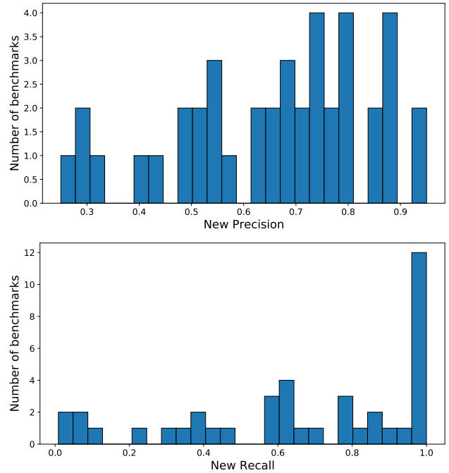
Figure 6: Precision and recall after call-graph pruning.
