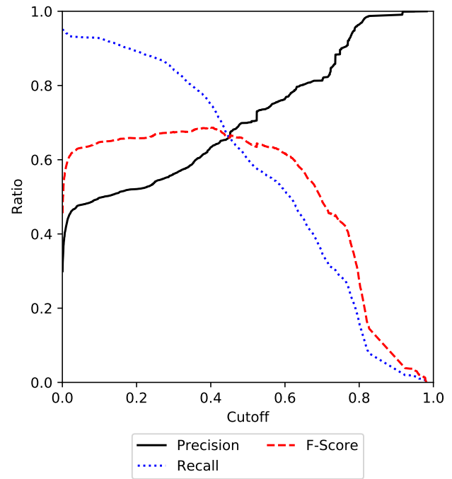
Figure 8: Probability cutoff plotted vs Precision, Recall and F-score curves for WALA
