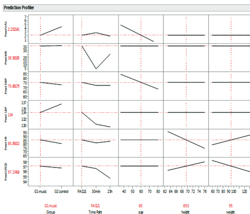
Figure 1. Prediction Profiler.
