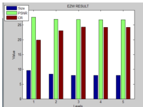
Fig.10. Result with EZW
