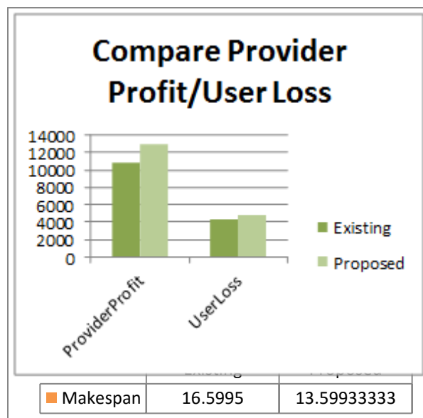
Fig. 2: Comparison b/w Provider profit and User loss of PSO
