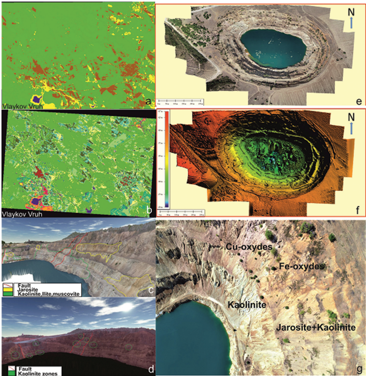
Fig. 1. a , Sentinel-2 image with classification of ore mineralisations; b , Aster image with classification of ore mineralisations; c , drone visual imaging overlaid on 3D generated model with detected mineral zones.; d , drone IR imaging overlaid on 3D denertated model with ground sample locations; e , VIS spectral range of Tsar Assen porphyry-copper deposit; f , IR spectral range of Tsar Assen porphyry-copper deposit; g , generated digital surface model with zones of mineralisation
