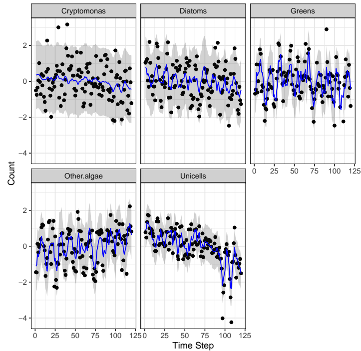
Fig. 10.6. Plot of the 2-state model fits to the phytoplankton data using ggplot.
