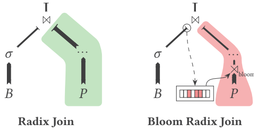
Figure 7: Bloom filters with selective joins. Tuples without a join partner are filtered early and are not materialized.
