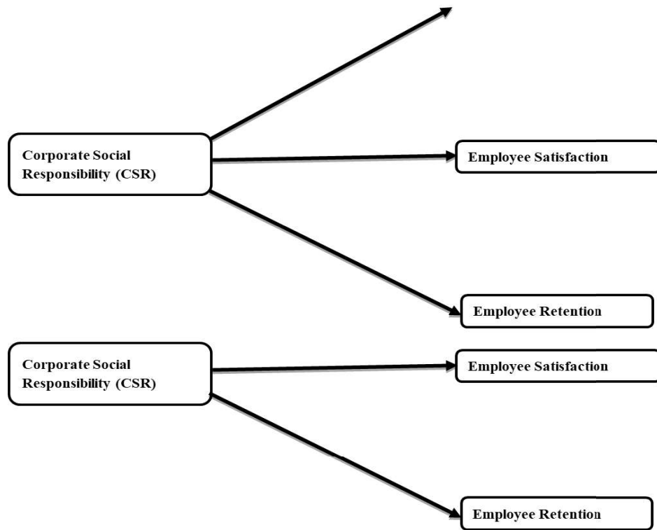
Figure 3.1 Theoretical Framework
