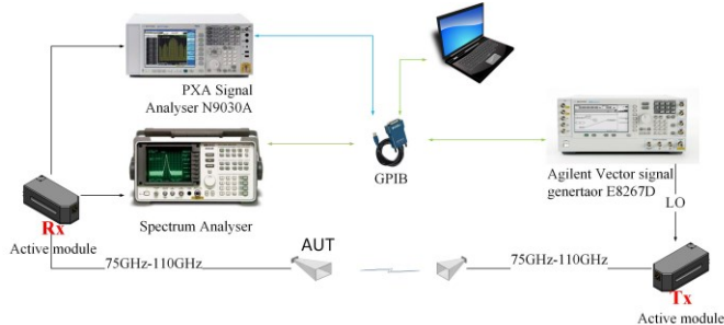
Fig. 10. Antenna measurement setup
