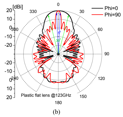
Fig. 3. 3D flat lens antenna theoretical performance: S-parameter (a) and Radiation pattern (b) at 122GHz
