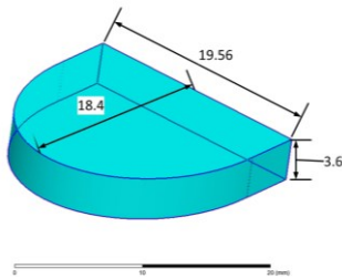
Fig. 2. 3D plastic flat lens antenna: theoretical HFSS model (dimensions are mm).
