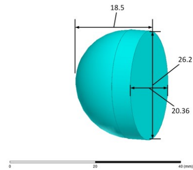
Fig. 4. 3D plastic lens antenna: theoretical HFSS model (dimensions are mm).
