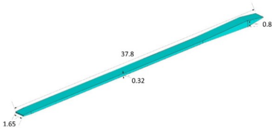
Fig. 6. Rod antenna: theoretical model (dimensions are mm).
