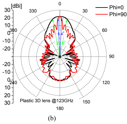
Fig. 5. 3D lens antenna theoretical performance: S-parameter (a) and Radiation pattern (b) at 122GHz
