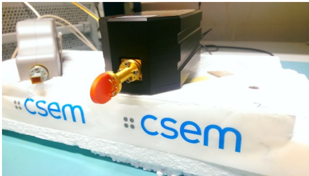
Fig. 11. 3D flat lens antenna attached the open end WG.
