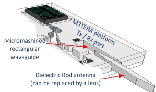
Fig. 1. M3TERA miniature mm-wave platform concept.
