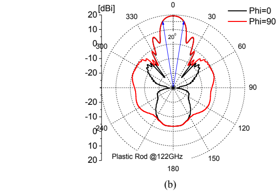
Fig. 7. Rod antenna theoretical results: S-parameters (a) and radiation pattern (b) at 122GHz.
