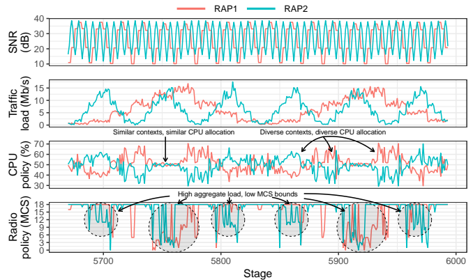
Fig. 21. vRAN with 2 vRAPs. \text{vrAIn} adapts the radio scheduling policy to minimize decoding errors (which are negligible and therefore not shown).
