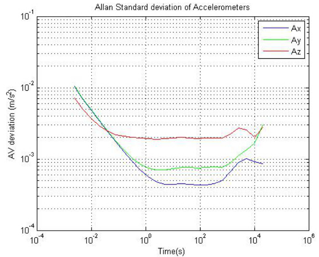
Figure 1: Allan variance for the EPSON accelerometers
