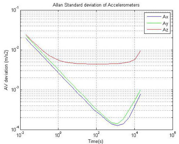
Figure 2: Allan variance for the MAXIM accelerometers
