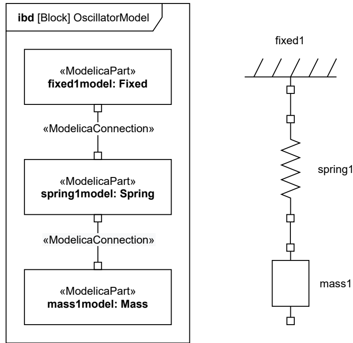
Figure 5 – Mass-damper system in SysML (left) and Modelica (right) formats. Figure reproduced from [28].
