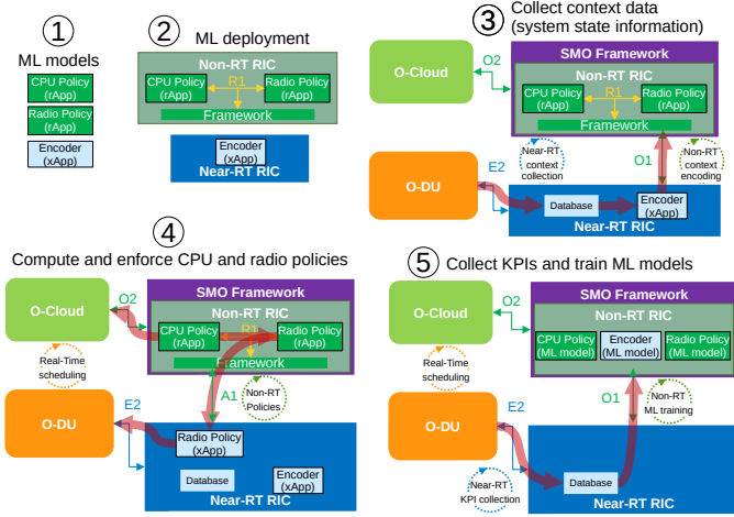
Fig. 5. Integration of an AI-aided vRAN resource orchestrator into O-RAN architecture.
