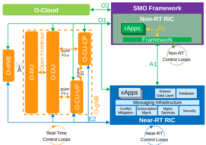
Fig. 1. O-RAN architecture [1]
