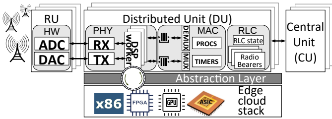
Fig. 4. O-Cloud at the edge serving shared computing resources to multiple O-DUs.
