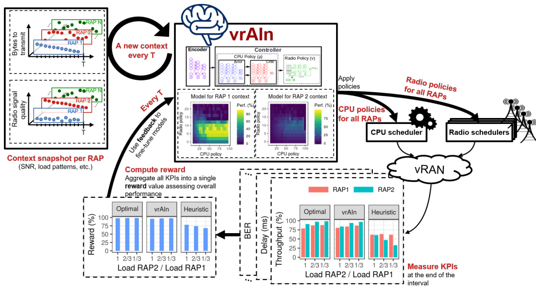
Fig. 3. AI-aided approach to joint computing/radio resource orchestration [4]
