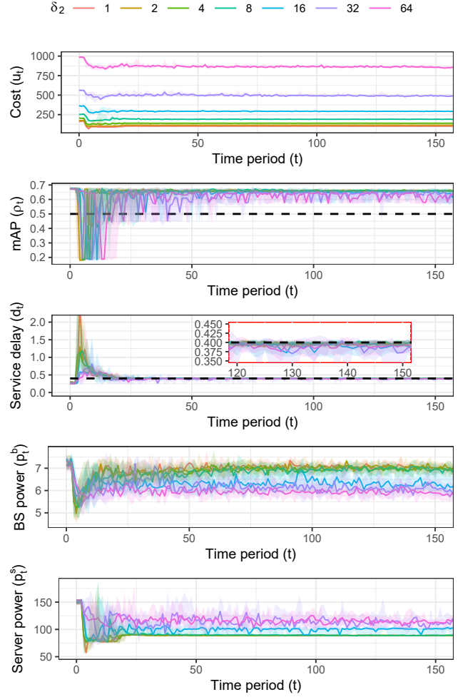
Figure 9: Convergence evaluation. A scenario with steady channel conditions (no context changes), \delta_1 = 1 mu/W, \rho^{min} = 0.5 , and d^{max} 0.4 s.
