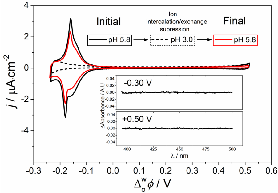
Fig. 4. Suppression and reactivation of the ZnPor membrane H-J interconversion monitored by CV and differential TIR-UV/vis absorbance. The scan rate for the CV was 5 \text{ mV}\cdot\text{s}^{-1} . Inset: differential absorbance of the membrane at pH 3.0 with \Delta_0^w \phi equal to -0.30 \text{ V} and +0.50 \text{ V} , respectively. The TIR-UV/vis absorbance spectrum at +0.50 \text{ V} was taken as the blank, and spectra at other \Delta_0^w \phi across the full potential range studied are shown in Fig. S12.
