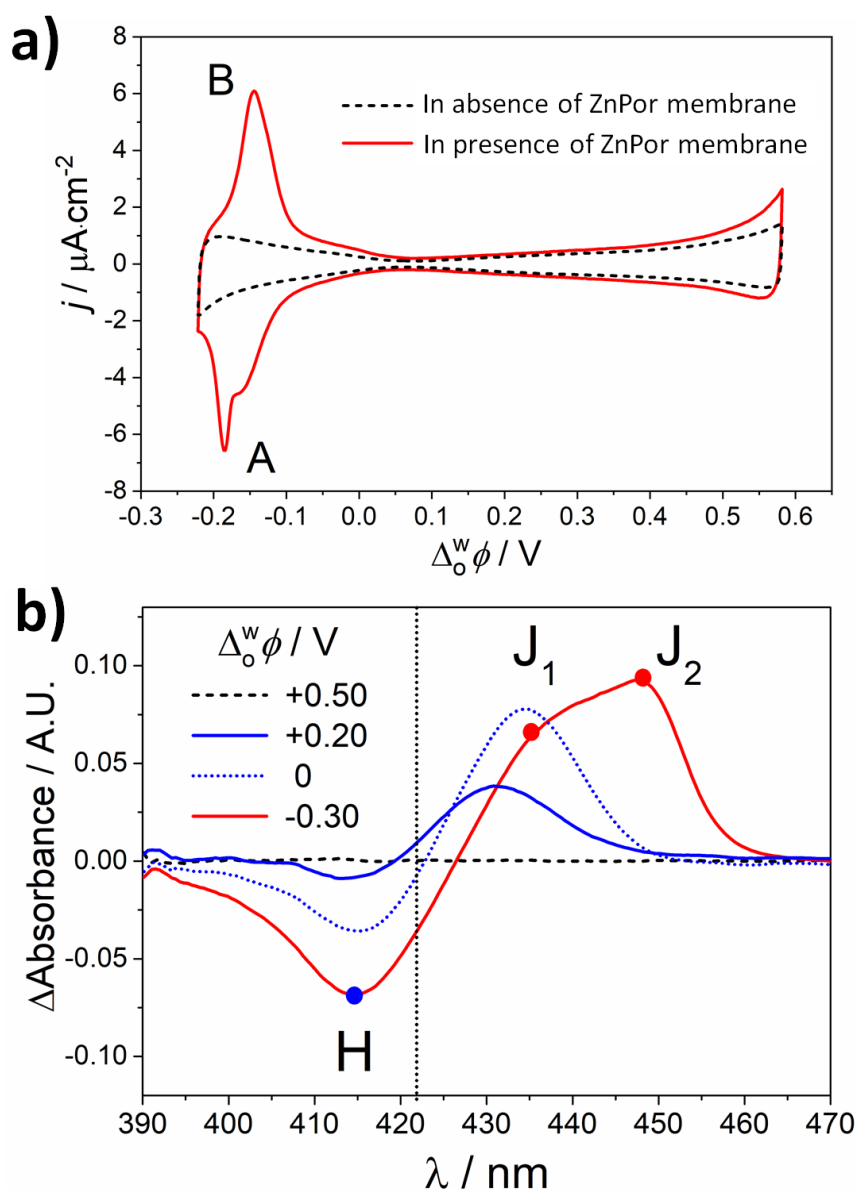
Fig. 2. (a) Cyclic voltammetry (CV) in the absence and presence of the ZnPor membrane in the configuration presented schematically in Fig. 1a. The scan rate was 25 \text{ mV}\cdot\text{s}^{-1} . The 4-electrode electrochemical cell setup used for these measurements is presented in Fig. S1. (b)
