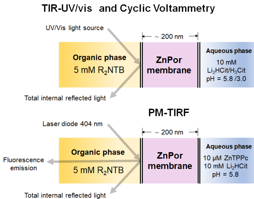
Fig. 1. Schematic configurations for spectroelectrochemical studies with the ZnPor membrane system. The techniques used were cyclic voltammetry (CV), in situ UV/vis absorbance and polarisation-modulation fluorescence spectroscopies in total internal reflection mode (TIR-UV/vis and PM-TIRF, respectively). The organic phase was \alpha,\alpha,\alpha -trifluorotoluene (TFT) containing 5 mM bis(triphenylphosphoranylidene)ammonium tetrakis(pentafluorophenyl)borate ( R_2NTB ). The aqueous phase was 10 mM lithium citrate ( Li_2HCit ) at pH 5.8, or 10 mM citric acid ( H_3Cit ) at pH 3.0. The ZnPor membrane was prepared from 10 \mu M solutions of ZnPor in contact with the TFT as described in the SI.
