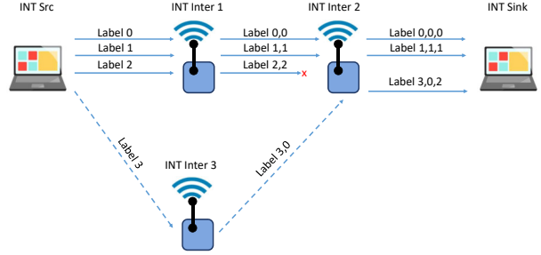
(b) Tracking reliability per hop in different paths.
