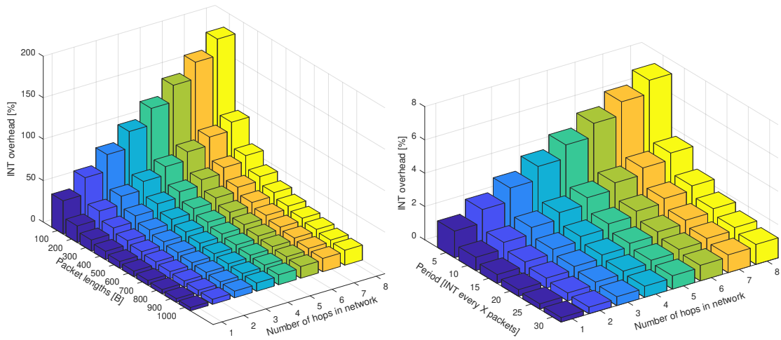
(a) Overhead vs different packet size and number of hops. (b) Overhead vs different packet period and number of hops. Fixed data packet size of 500B.
