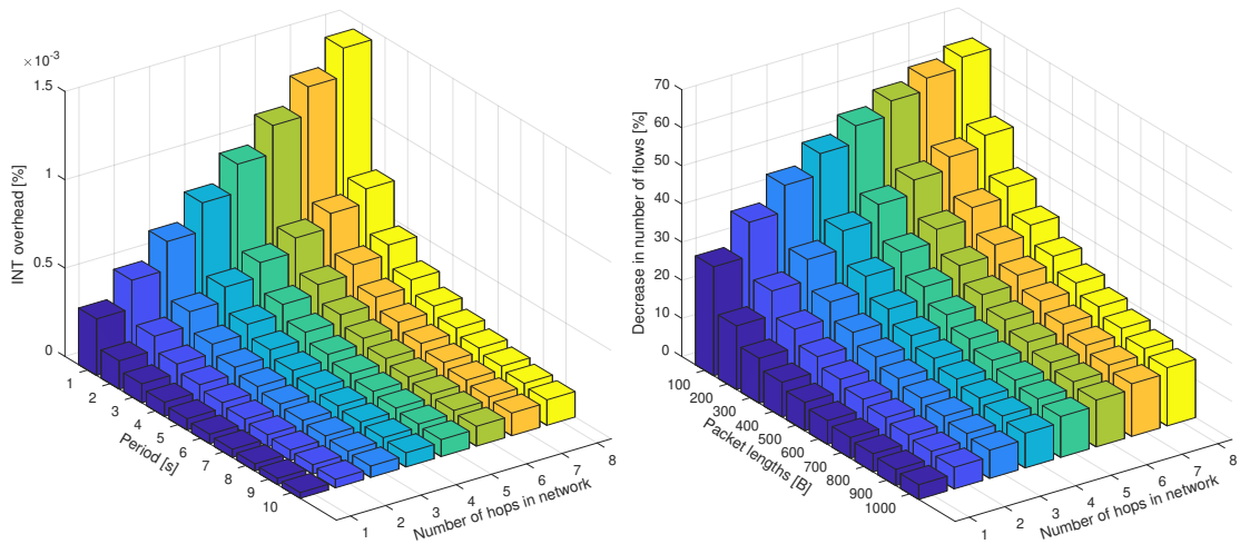
(c) Overhead vs different INT period and number of hops. Fixed data rate of 100Mbps. (d) Decrease in number of flows vs different data packet length and number of hops.
