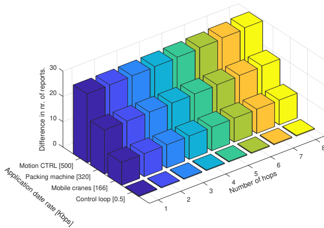
Fig. 8. Difference between number of INT reports and active probing reports for different application requirements [2] keeping the number of channel access requirements the same for data packets.
