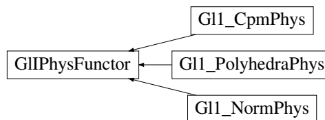
Fig. 2.43: Inheritance graph of GlPhysFuncor . See also: Gl1_CpmPhys , Gl1_NormPhys , Gl1_PolyhedraPhys .
