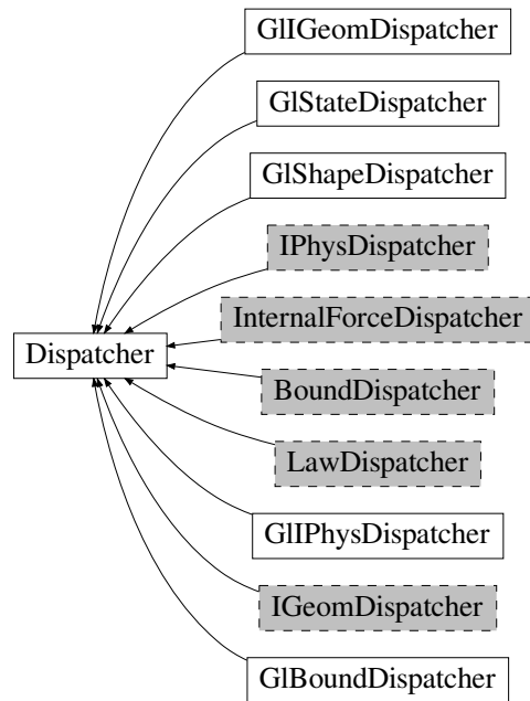
Fig. 2.31: Inheritance graph of Dispatcher, gray dashed classes are discussed in their own sections: IPhysDispatcher , InternalForceDispatcher , BoundDispatcher , LawDispatcher , IGeomDispatcher . See also: GIBoundDispatcher , GIIGeomDispatcher , GIIPhysDispatcher , GIShapeDispatcher , GIStateDispatcher .
