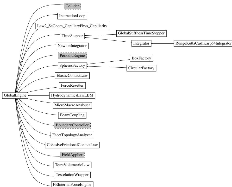
Fig. 2.25: Inheritance graph of GlobalEngine, gray dashed classes are discussed in their own sections: Collider , PeriodicEngine , BoundaryController , FieldApplier . See also: BoxFactory , CircularFactory , CohesiveFrictionalContactLaw , ElasticContactLaw , FEInternalForceEngine , FacetTopologyAnalyzer , FoamCoupling , ForceResetter , GlobalStiffnessTimeStepper , HydrodynamicsLawLBM , Integrator , InteractionLoop , Law2_ScGeom_CapillaryPhys_Capillarity , MicroMacroAnalyser , NewtonIntegrator , RungeKuttaCashKarp54Integrator , SpheresFactory , TesselationWrapper , TetraVolumetricLaw , TimeStepper .
