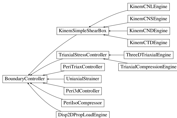
Fig. 2.27: Inheritance graph of BoundaryController. See also: Disp2DPropLoadEngine , KinemCNDEngine , KinemCNLEngine , KinemCNSEngine , KinemCTDEngine , KinemSimpleShearBox , Peri3dController , PeriIsoCompressor , PeriTriaxController , ThreeDTriaxialEngine , TriaxialCompressionEngine , TriaxialStressController , UniaxialStrainer .
