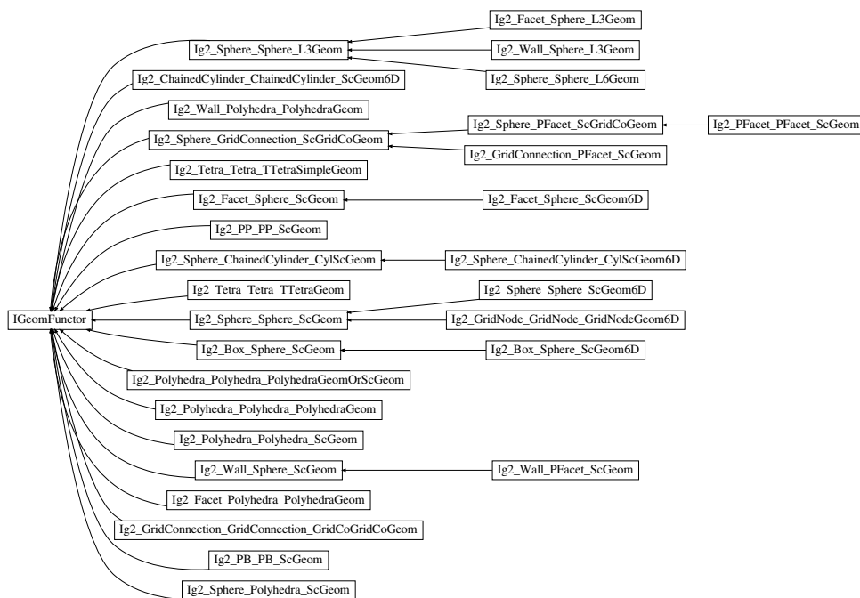
Fig. 2.34: Inheritance graph of IGeomFuncator. See also: Ig2_Box_Sphere_ScGeom , Ig2_Box_Sphere_ScGeom6D , Ig2_ChainedCylinder_ChainedCylinder_ScGeom6D , Ig2_Facet_Polyhedra_PolyhedraGeom , Ig2_Facet_Sphere_L3Geom , Ig2_Facet_Sphere_ScGeom , Ig2_Facet_Sphere_ScGeom6D , Ig2_GridConnection_GridConnection_GridCoGridCoGeom , Ig2_GridConnection_PFacet_ScGeom , Ig2_GridNode_GridNode_GridNodeGeom6D , Ig2_PB_PB_ScGeom , Ig2_PFacet_PFacet_ScGeom , Ig2_PP_PP_ScGeom , Ig2_Polyhedra_Polyhedra_PolyhedraGeom , Ig2_Polyhedra_Polyhedra_PolyhedraGeomOrScGeom , Ig2_Polyhedra_Polyhedra_ScGeom , Ig2_Sphere_ChainedCylinder_CylScGeom , Ig2_Sphere_ChainedCylinder_CylScGeom6D , Ig2_Sphere_GridConnection_ScGridCoGeom , Ig2_Sphere_PFacet_ScGridCoGeom , Ig2_Sphere_Polyhedra_ScGeom , Ig2_Sphere_Sphere_L3Geom , Ig2_Sphere_Sphere_L6Geom , Ig2_Sphere_Sphere_ScGeom , Ig2_Sphere_Sphere_ScGeom6D , Ig2_Tetra_Tetra_TTetraGeom , Ig2_Tetra_Tetra_TTetraSimpleGeom , Ig2_Wall_PFacet_ScGeom , Ig2_Wall_Polyhedra_PolyhedraGeom , Ig2_Wall_Sphere_L3Geom , Ig2_Wall_Sphere_ScGeom .
