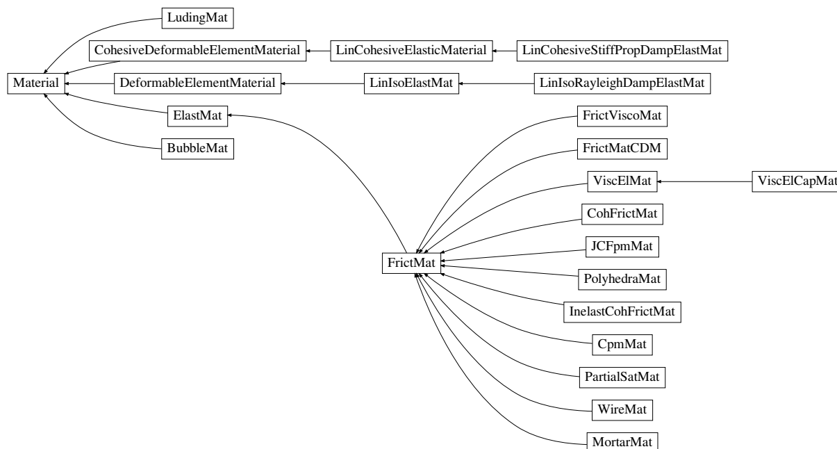
Fig. 2.21: Inheritance graph of Material. See also: BubbleMat , CohFrictMat , CohesiveDeformableElementMaterial , CpmMat , DeformableElementMaterial , ElastMat , FrictMat , FrictMatCDM , FrictViscoMat , InelastCohFrictMat , JCFpmMat , LinCohesiveElasticMaterial , LinCohesiveStiffPropDampElastMat , LinIsoElastMat , LinIsoRayleighDampElastMat , LudingMat , MortarMat , PartialSatMat , PolyhedraMat , ViscElCapMat , ViscElMat , WireMat .
