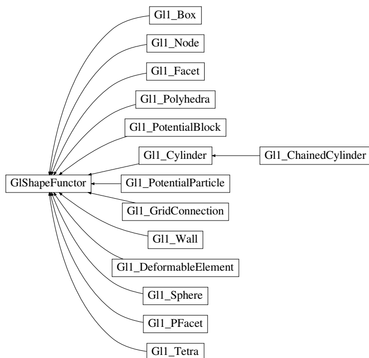
Fig. 2.40: Inheritance graph of GIShapeFuncor. See also: GI1_Box , GI1_ChainedCylinder , GI1_Cylinder , GI1_DeformableElement , GI1_Facet , GI1_GridConnection , GI1_Node , GI1_PFacet , GI1_Polyhedra , GI1_PotentialBlock , GI1_PotentialParticle , GI1_Sphere , GI1_Tetra , GI1_Wall .
