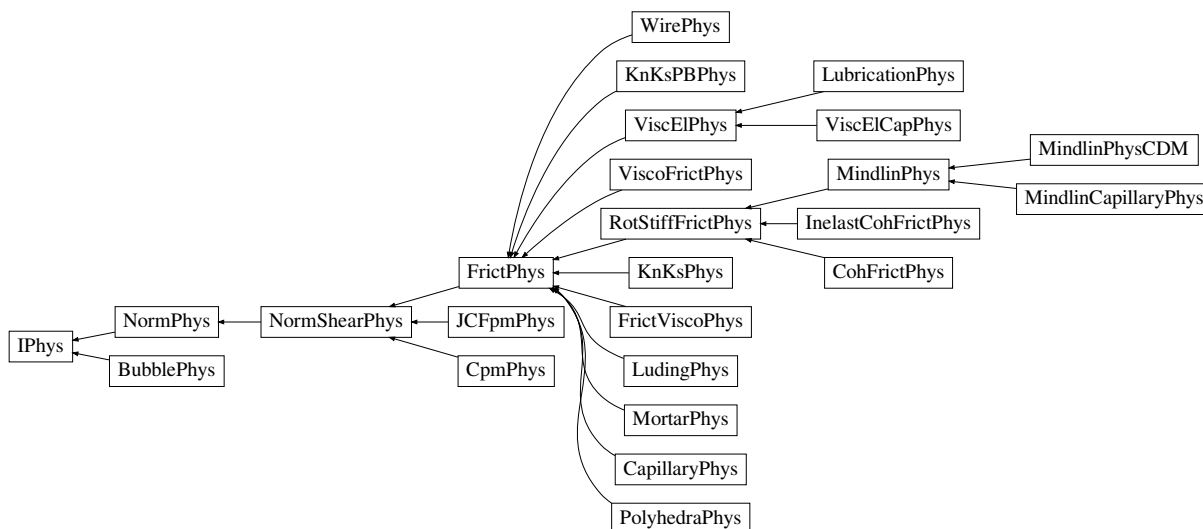
Fig. 2.24: Inheritance graph of IPhys . See also: BubblePhys , CapillaryPhys , CohFrictPhys , CpmPhys , FrictPhys , FrictViscoPhys , InelastCohFrictPhys , JCFpmPhys , KnKsPBPhys , KnKsPhys , LubricationPhys , LudingPhys , MindlinCapillaryPhys , MindlinPhys , MindlinPhysCDM , MortarPhys , NormPhys , NormShearPhys , PolyhedraPhys , RotStiffFrictPhys , ViscElCapPhys , ViscElPhys , ViscoFrictPhys , WirePhys .
