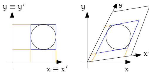
Fig. 2.7: Constructing axis-aligned bounding box ( Aabb ) of a sphere in simulation space coordinates (without periodic cell – left) and transformed cell coordinates (right), where collision detection axes x' , y' are not identical with simulation space axes x , y . Bounds' projection to axes is shown by orange lines.
