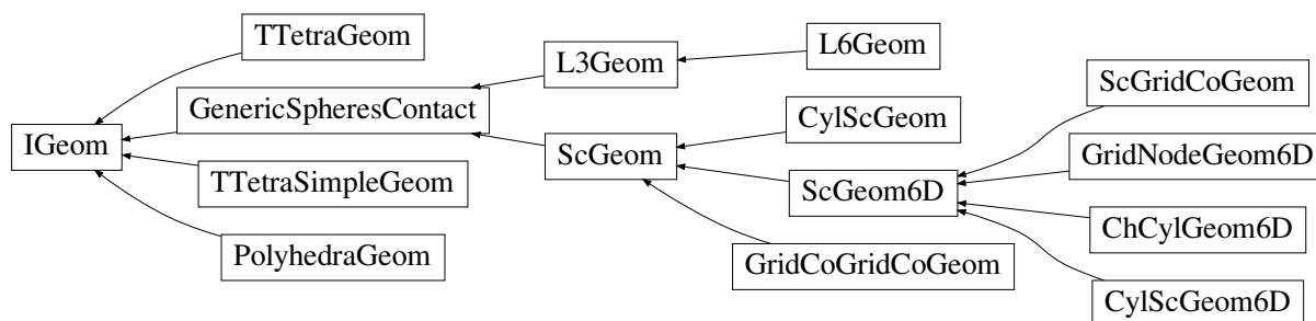
Fig. 2.23: Inheritance graph of IGeom . See also: ChCylGeom6D , CylScGeom , CylScGeom6D , GenericSpheresContact , GridCoGridCoGeom , GridNodeGeom6D , L3Geom , L6Geom , PolyhedraGeom , ScGeom , ScGeom6D , ScGridCoGeom , TTetraGeom , TTetraSimpleGeom .
