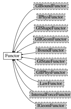
Fig. 2.32: Inheritance graph of Functor, gray dashed classes are discussed in their own sections: GIBoundFunctor , IPhysFunctor , GShapeFunctor , GIGeomFunctor , BoundFunctor , GIStateFunctor , GIIPhysFunctor , LawFunctor , InternalForceFunctor , IGeomFunctor .
