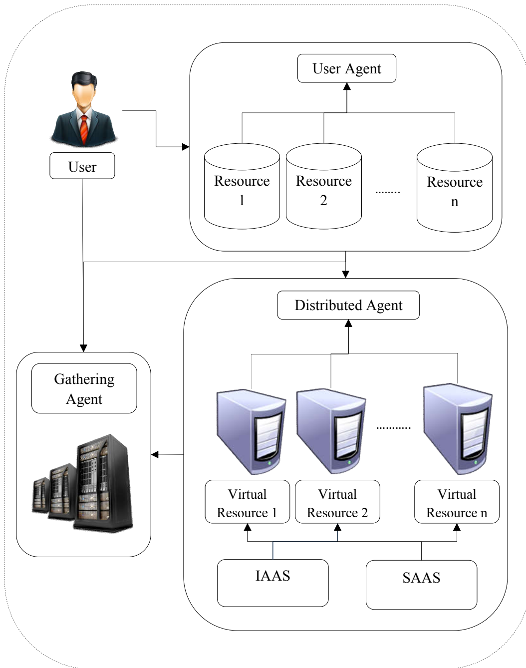
Figure1.1: IMAV (Intelligent Multi-Agent Model for Resource Virtualization)
