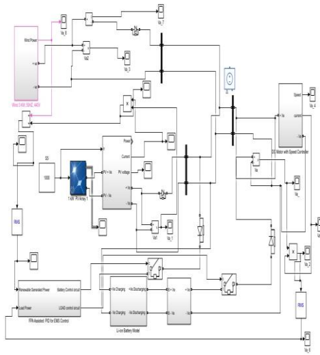
Fig.6 Proposed PV-WT HRES EMS control model
