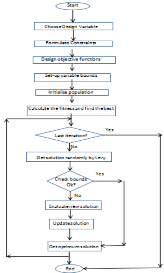
Fig.5 Workflow of FPA algorithm
