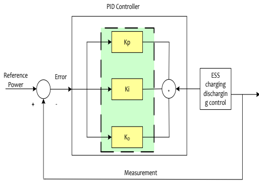
Fig 3. PID Controller for EMS control
