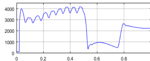
Fig. 11. Load side demand variations with FPA-EMS
