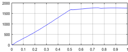
Fig. 12. Speed control variation with FPA-EMS
