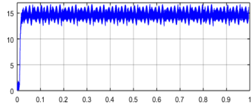
Fig. 8 WT -RES current (A) generated with FPA-EMS control
