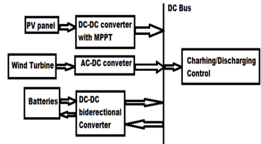
Fig. 1. PV-WT HRES power grid design
