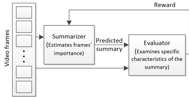
Fig. 6. High-level representation of the analysis pipeline of supervised algorithms that learn summarization based on hand-crafted rewards and reinforcement learning.
