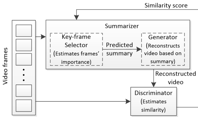
Fig. 5. High-level representation of the analysis pipeline of unsupervised algorithms that learn summarization by increasing the similarity between the summary and the video.
