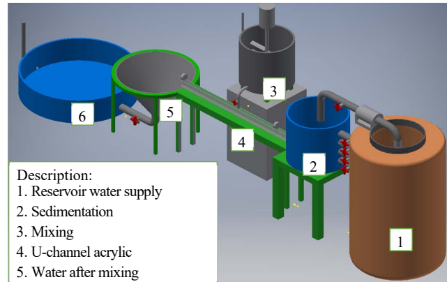
Fig. 2. Research installation
