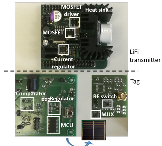
Figure 1: PassiveLiFi: hardware prototypes of LiFi transmitter and passive tag. The tag comprises LiFi module for downlink (backside), solar cell array for energy harvesting and downlink communication (frontside), and RF backscatter module for uplink.
