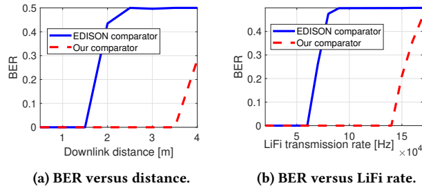
(a) BER versus distance. (b) BER versus LiFi rate. Figure 18: Threshold circuit evaluation: BER versus distance (at 50 kHz of LiFi transmission rate) and BER versus LiFi transmission rate (at a distance of 1.5 m) with 800 lux background light.
