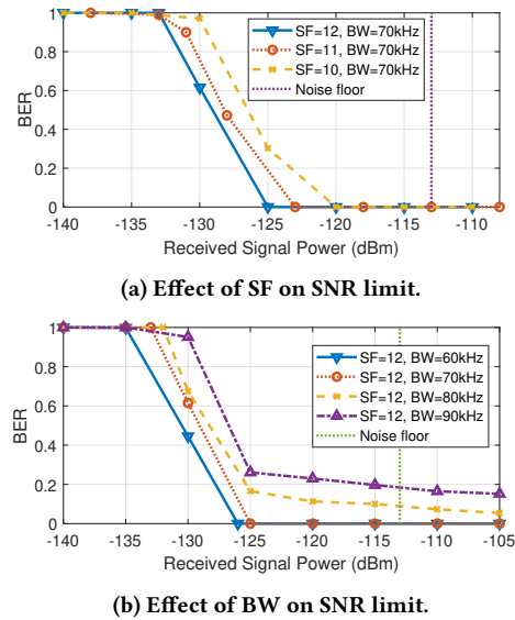
(a) Effect of SF on SNR limit. (b) Effect of BW on SNR limit. Figure 19: Evaluation of backscatter receiver to detect chirps below the noise floor.
