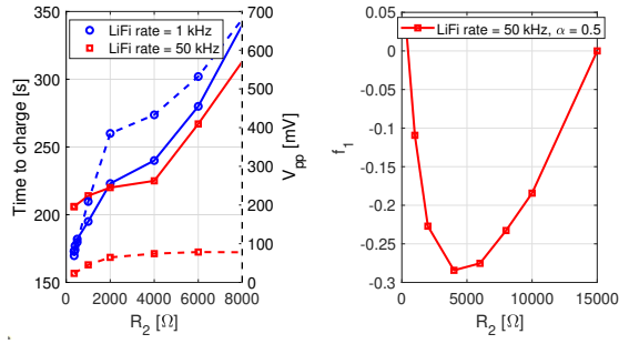
(a) Peak-to-peak voltage (dashed) and Time to charge (solid) for different R_2 values and LiFi rates. (b) The optimal point for both communication and harvesting is R_2 = 4 k \Omega , when LiFi rate = 50 kHz.
