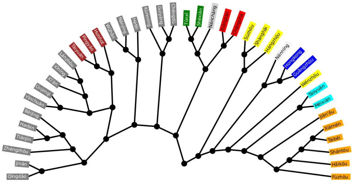
C: Neighbor-Joining
