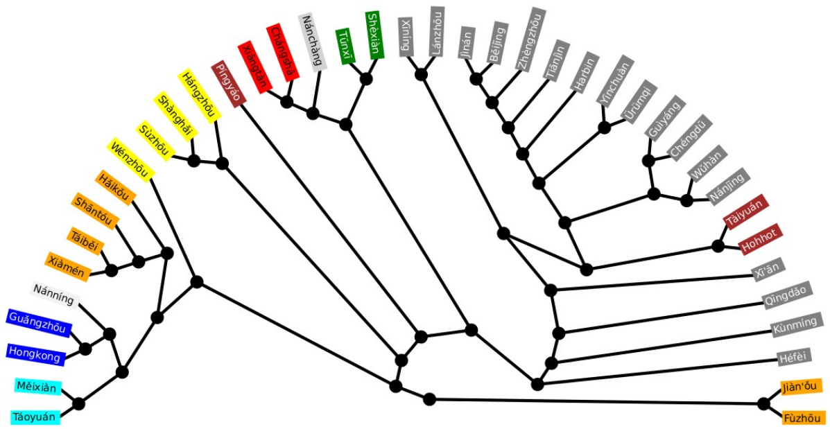
C: Neighbor-Joining
