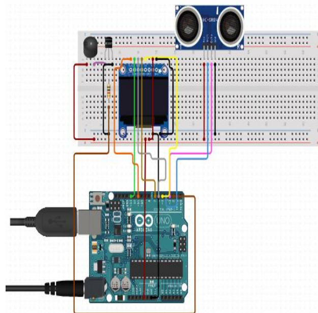
Fig 6. Circuit Diagram
