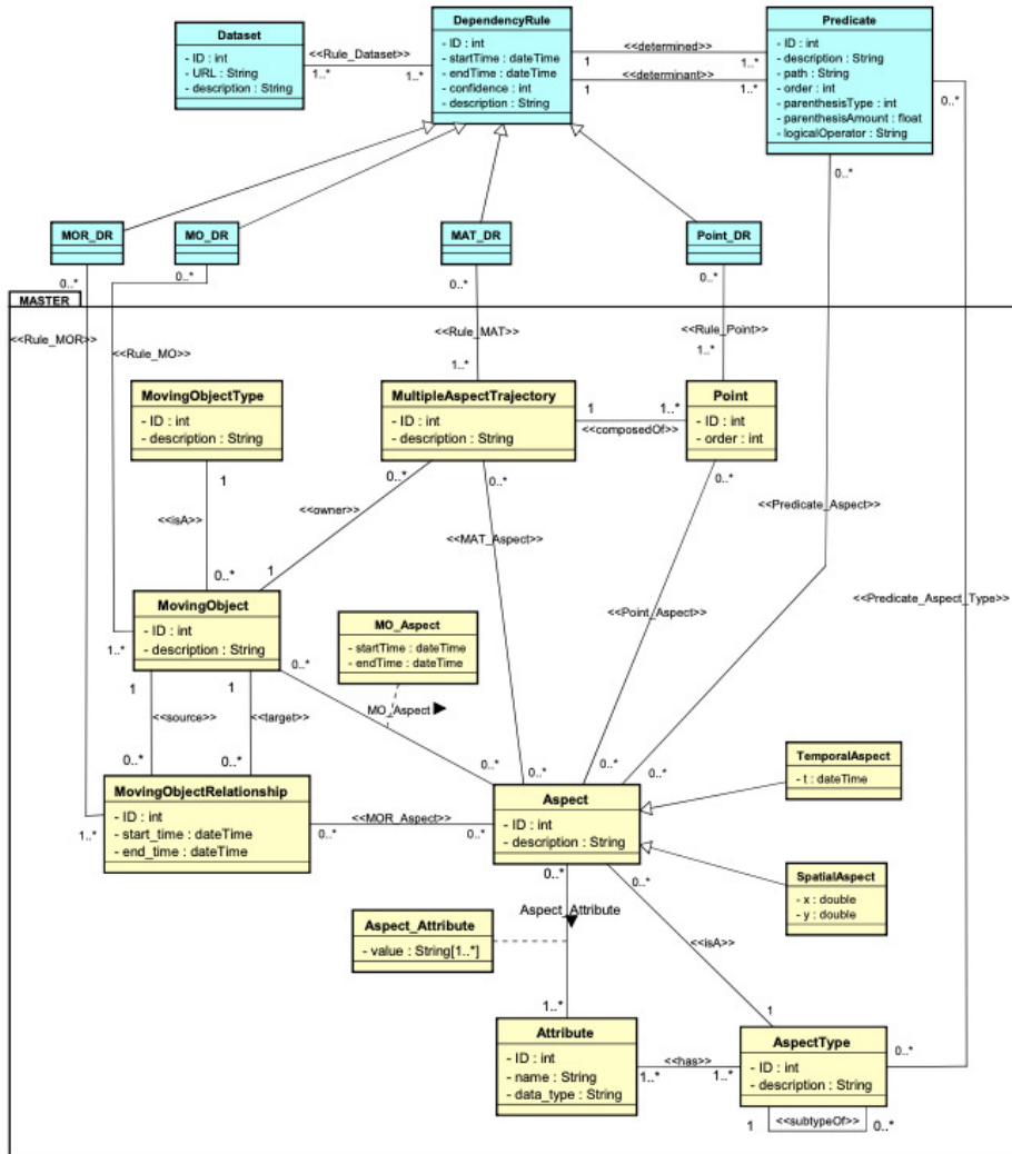
Fig. 1. The MASTER conceptual model and the dependency rule extension
