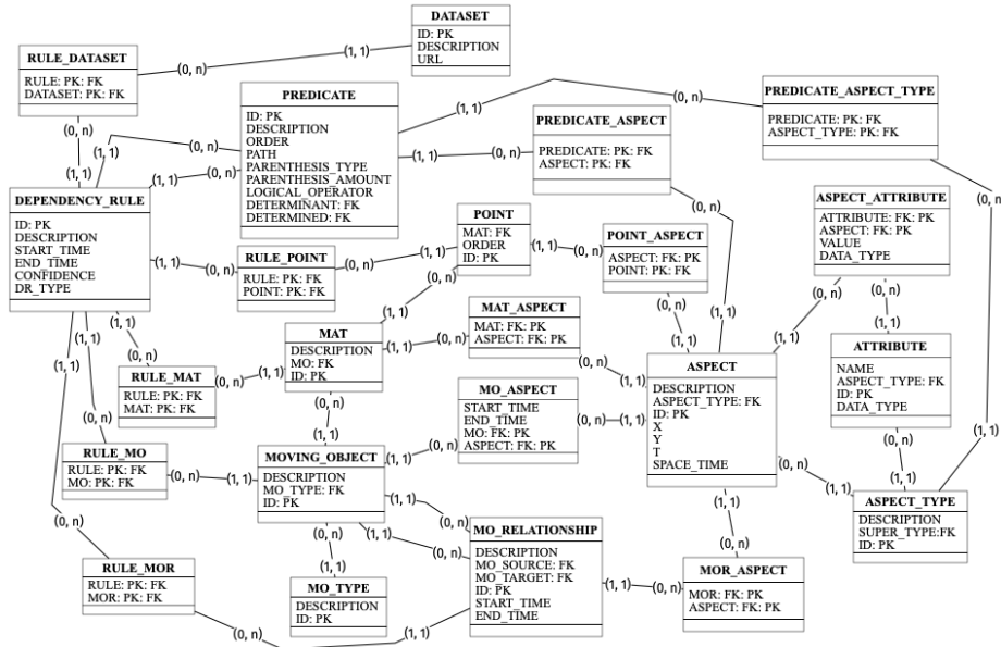
Fig. 2. A relational schema for MASTER DR
