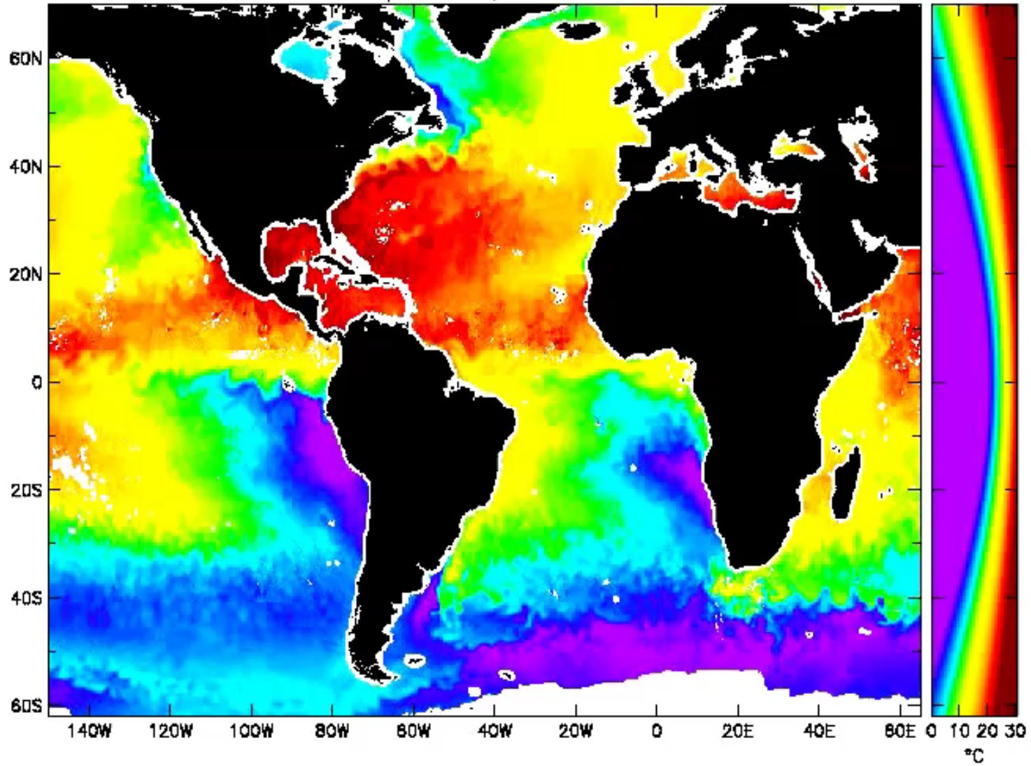
AMSR-E Sea Surface Temperature, 1 October 2002
