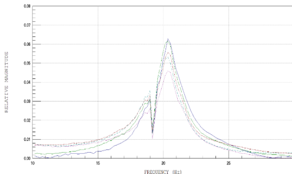
Fig. 8. The First Natural frequency with 50 kg load and 60° angle
