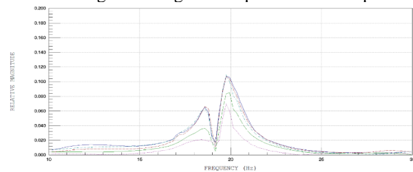
Fig. 4. Natural frequency with 50 kg load and Operator A
