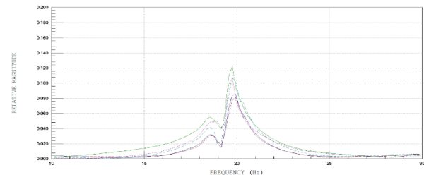
Fig. 3. Natural frequency in one quarter of the cable span
