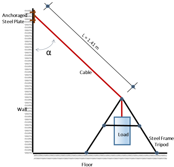
Fig. 1. Experiment set-up
