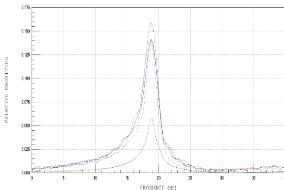
Fig. 7. The First Natural frequency with 50 kg load and 45° angle
