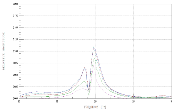
Fig. 6. Natural frequency with 50 kg load and 30° angle
