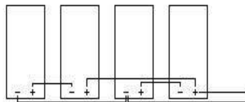
Two 12v/3.5A panels in series and two in parallel. This doubles the voltage and doubles the amps to make 24 volts and 7 amps.
