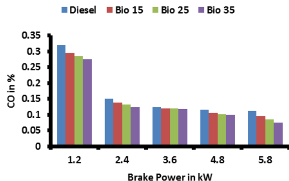
Fig.6. Brake Power vs CO emission
