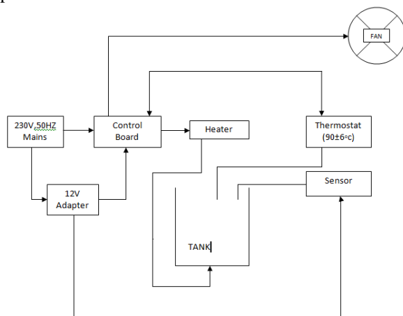
Fig: 3.1 Block Diagram
