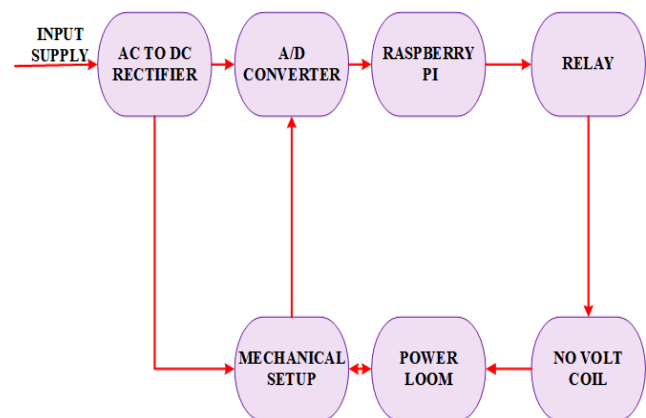
Figure.4.1. Block Diagram of the proposed power loom control
