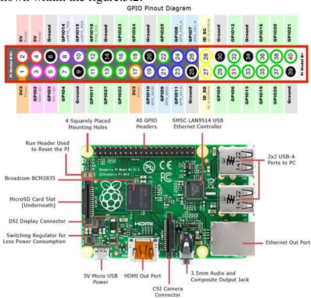
Figure.5.2.Hardware Specifications of Raspberry pi
