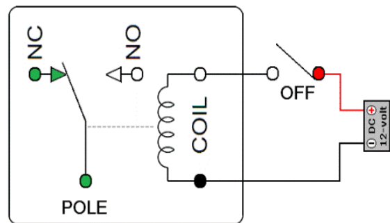
Figure.5.3.Relay Model
