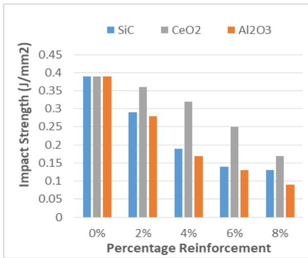
Fig 8 Variation of Impact Strength with increased contents of reinforcement of cold extruded matrix Al6061 alloy & its composite systems.
