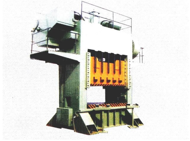
Fig.2 Photograph of Mechanical press used in the present work
