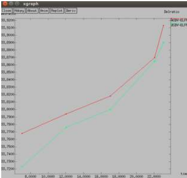
Figure 13. Graph of Time Vs Delay w.r.t. Table 1.2 and 1.3
