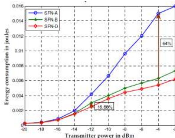
Figure 1. Energy consumption Vs Transmitter power
