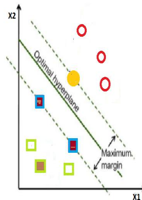
Fig. 3. SVM for linearly separable data
