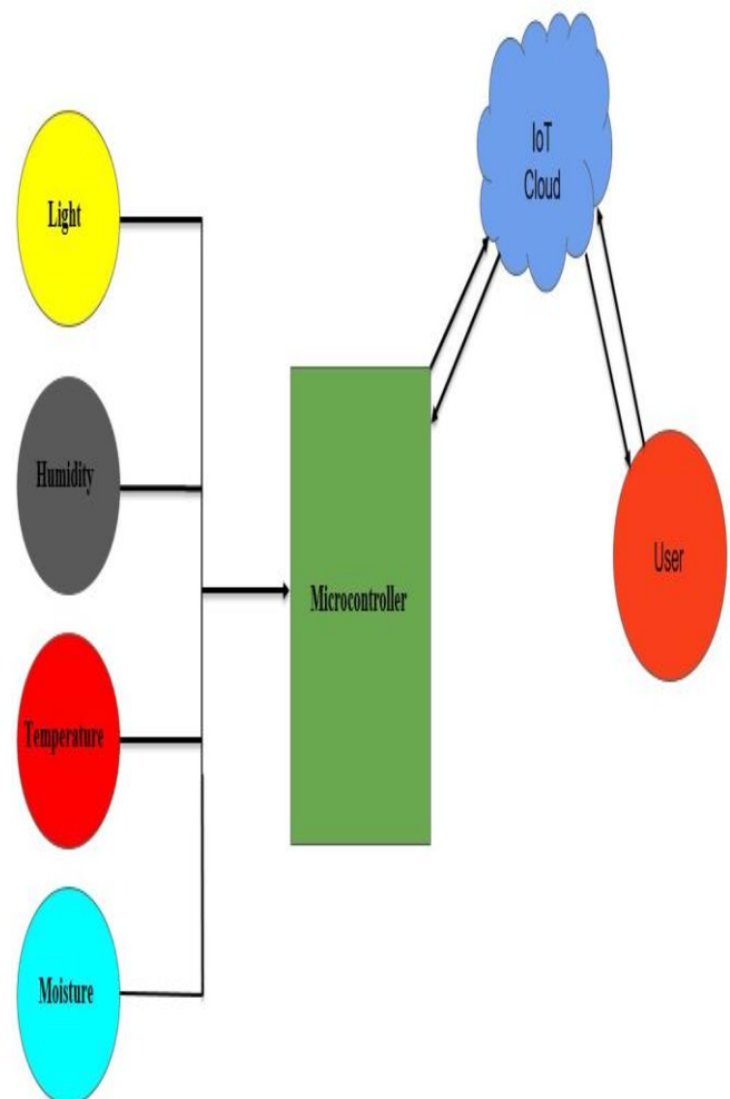
Fig. 1. Basic Block Diagram of the system
