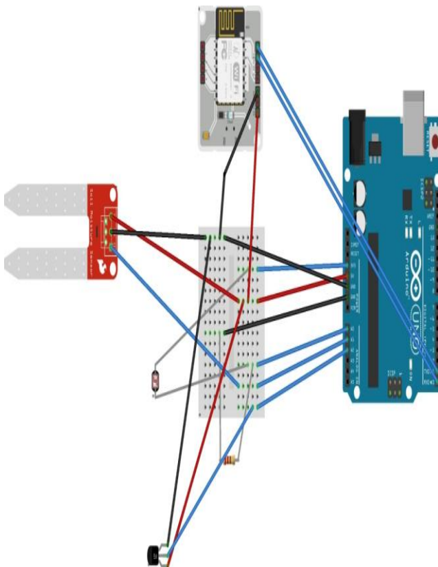
Fig. 2. Connection Diagram of the system
