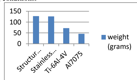
Fig. 6. Weight comparison
