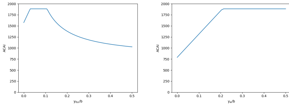
(a) Sensitivity to the lateral position of the fuselage-mounted rotors. (b) Sensitivity to the lateral position of the wing-mounted rotors.
