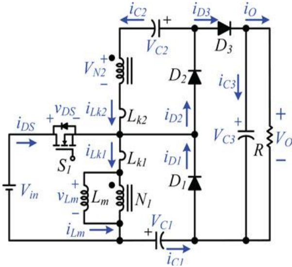
Figure3: Polarity definitions of voltage and current in proposed converter
