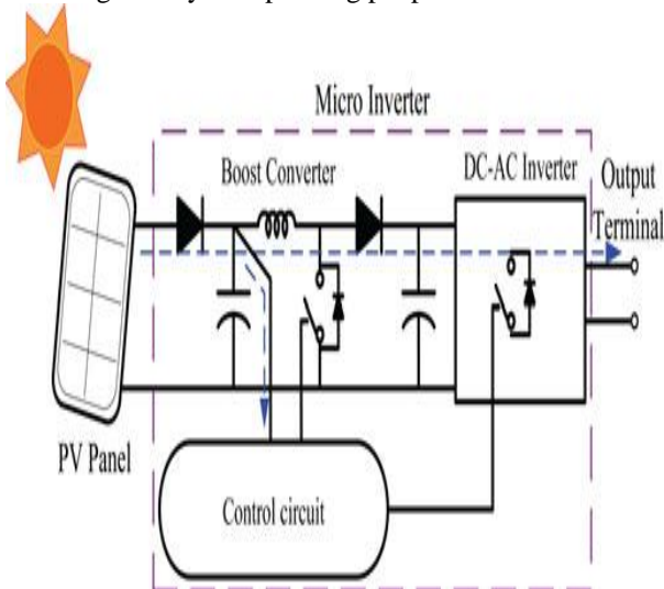
Figure2: Potential difference on the output terminal of non floating switch Micro inverter
