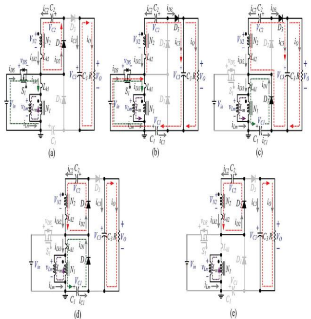
Figure5: CCM operation modes
