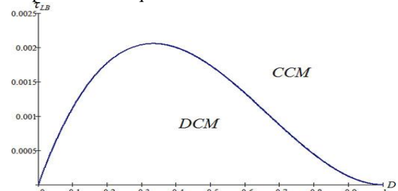
Figure7: Boundary condition of \tau_{LB} of proposed converter under n = 5
