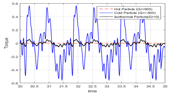
Fig.3. Torque of particles with respect to time
