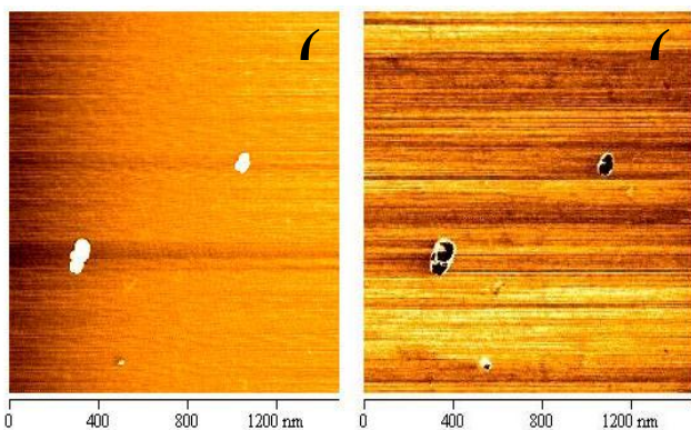
Figure 5 (a) Topography and (b) Phase images of scan size 1300 nm of drug, polymer loaded magnetite nanoparticles (concentration of magnetite is 25 µl)
