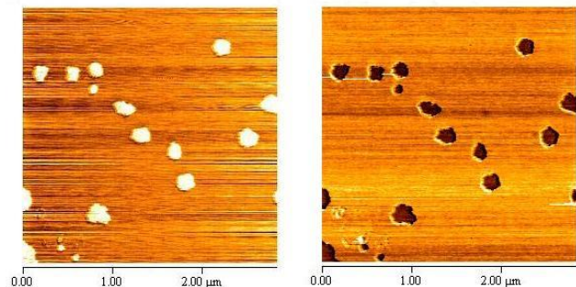
Figure 2 (a) Topography and (b) phase images of scan size 3 \mu\text{m} of magnetite nanoparticles coated with chitosan for a coating duration of 4 hours
