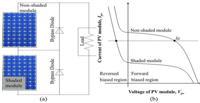
Fig. 1 (a) PV array under partial shading conditions. (b) P-V curve of PV Modules
